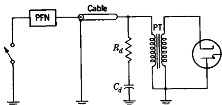
FIG. 10-14.—Line-type pulser with a despiking RC -network.
